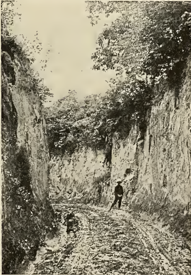
FIG. 62.—A road through a deposit of deep loess along the lower Illinois River. The deposit is 30 to 50 feet deep. The vertical walls are characteristic.
